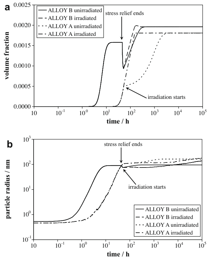
Fig. 7. Comparison of inter-granular Fe 3 C precipitation in high Ni/high Cu (ALLOY B) and high Ni/low Cu (ALLOY A) with and without irradiation. Note that the scale on the volume fraction curve is larger than for similar curves for ALLOY B (e.g., Fig. 5) showing both the effects of irradiation and Cu content.
