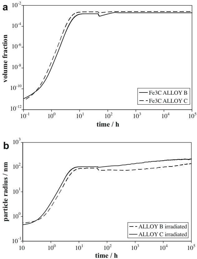
Fig. 6. Comparison of predicted Fe 3 C precipitation in alloys ALLOY B (high Ni/high Cu and ALLOY C (low Ni/high Cu) under irradiation conditions showing the effects of Ni content.
