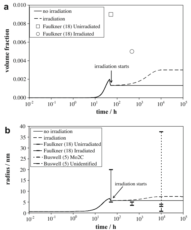
Fig. 4. Simulated volume fraction (a) and particle size (b) of intra-granular Mo 2 C in ALLOY B (high Ni/high Cu) compared with measurements reported by Buswell [5] and Faulkner [18].
