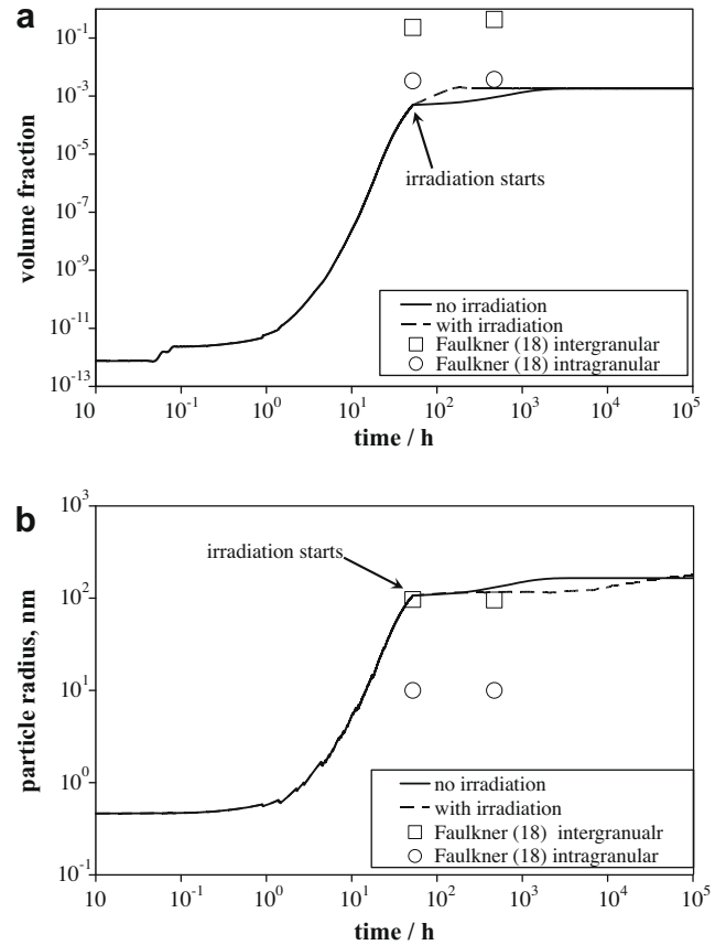
Fig. 2. Comparison of measured (symbols) and predicted (lines) \text{Fe}_3\text{C} precipitation in high Ni/low Cu (ALLOY A) alloy: (a) volume fraction of particles; (b) mean particle size.
