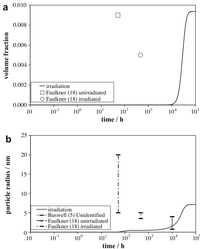
Fig. 3. Simulated volume fraction (a) and particle size (b) of intra-granular Cu-rich particles in ALLOY B compared with measurements of small unidentified particles reported by Buswell [5] and Faulkner [18] showing the formation of these particles are the effects of irradiation-enhanced diffusion.
