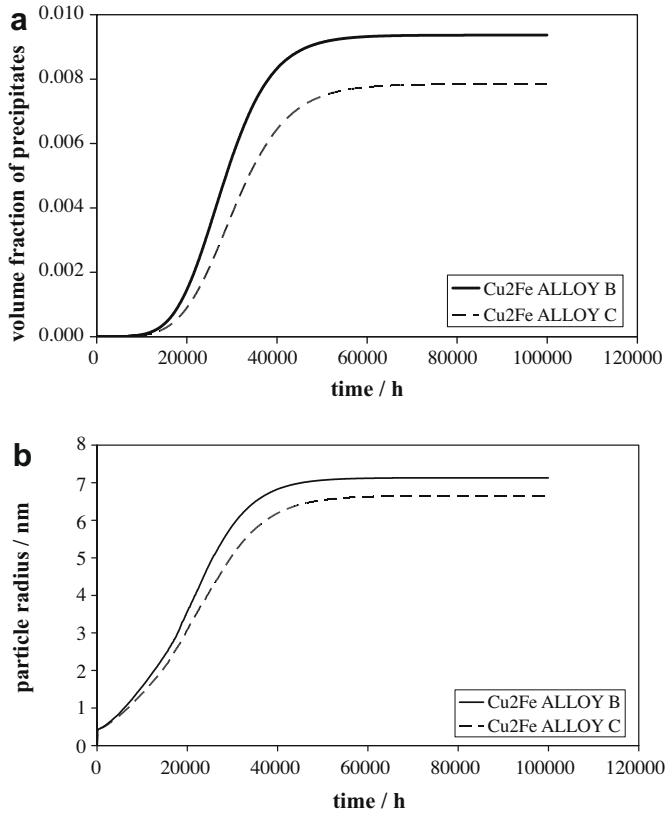
Fig. 5. Comparison of predicted Cu-rich precipitation in alloys ALLOY B (high Ni/high Cu with ALLOY C (low Ni/high Cu) showing the effects of Ni content.
