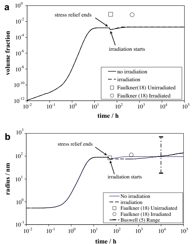
Fig. 1. Simulated volume fraction (a) and particle size (b) of inter-granular Fe 3 C in ALLOY B (lines) compared with measurements of Faulkner [18] and Buswell [5] (symbols) showing reasonable agreement between simulation and experimental results.
